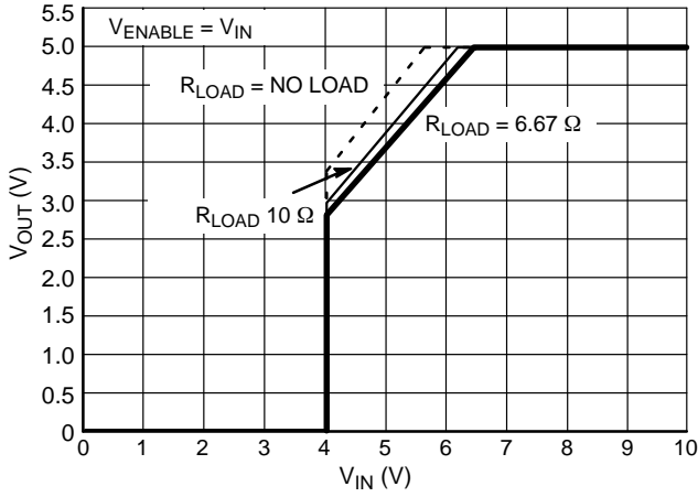
Figure 2. V_{OUT} vs. V_{IN} over R_{LOAD} ; T = 25^{\circ}C
